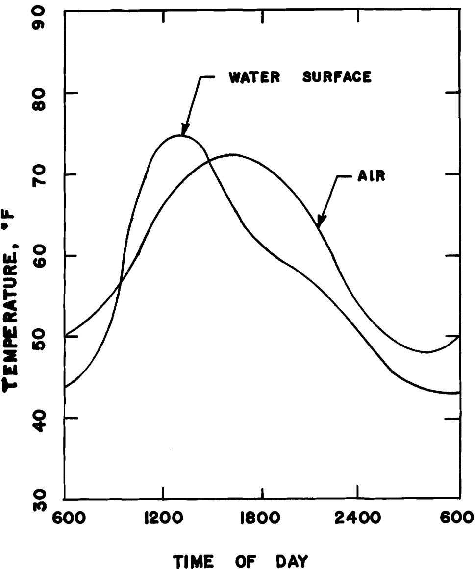
Figure 3. Temperatures for a Winter Day.
