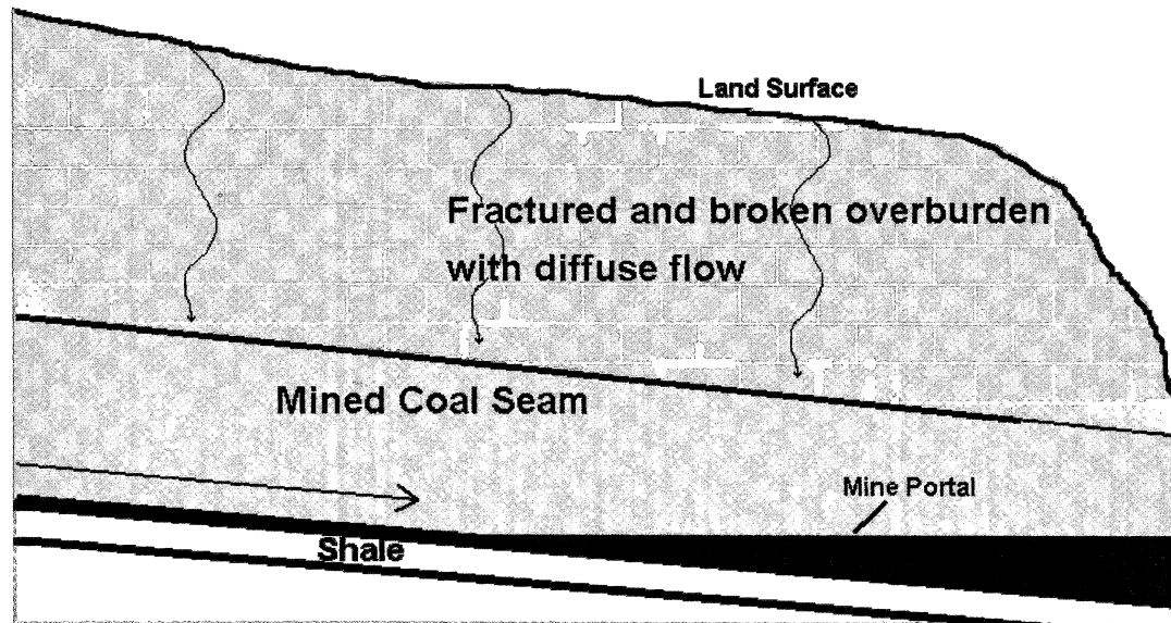
Figure 4. Conceptualized Flow System Within the Mine Aquifer System.
