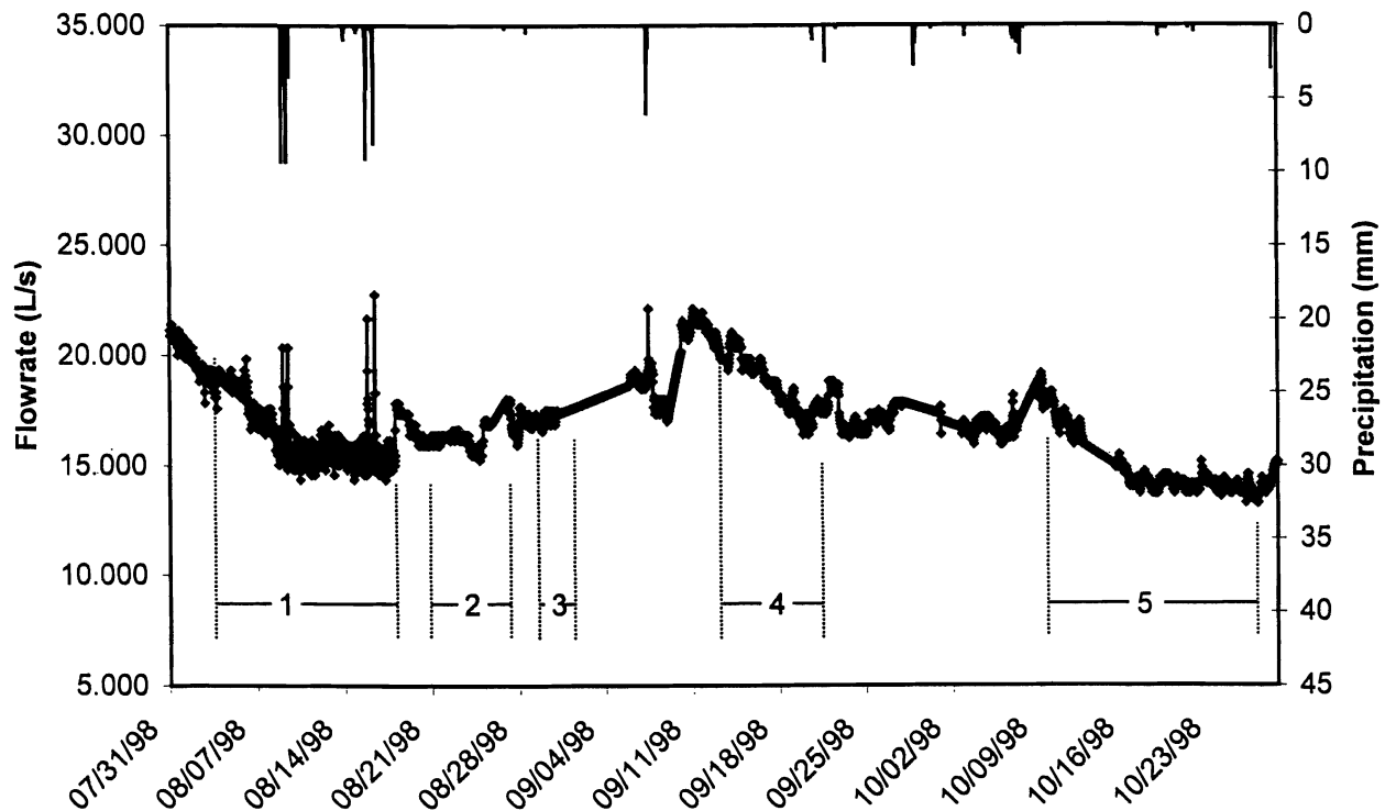
Figure 3. Hydrograph and Precipitation Data Showing Recession periods (numbered).
