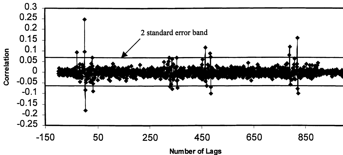
Figure 6. Cross-Correlation Data Obtained From 30-Minute Time Intervals.
