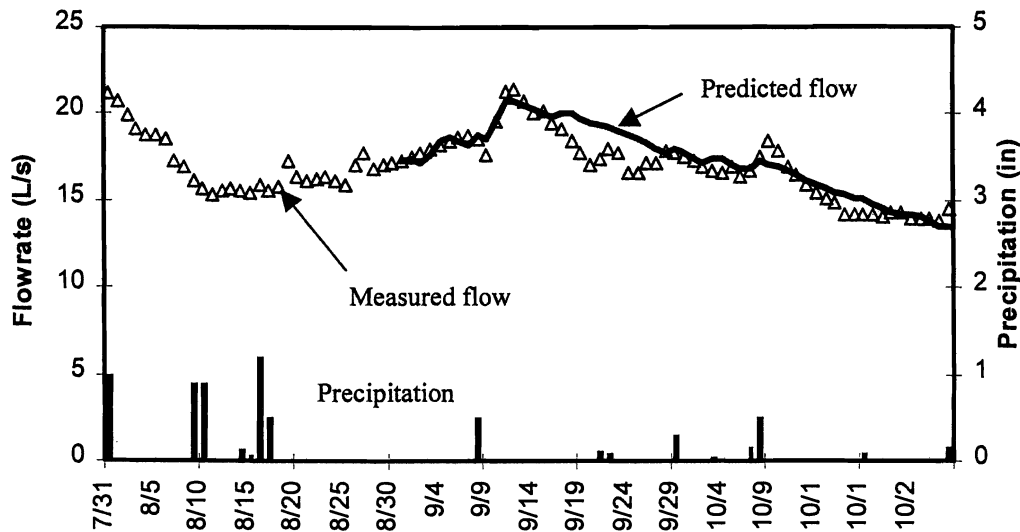
Figure 8. Predicted Flow Rates From Model Results Compared With Measured Flow Rates for One-Day Time Intervals.
