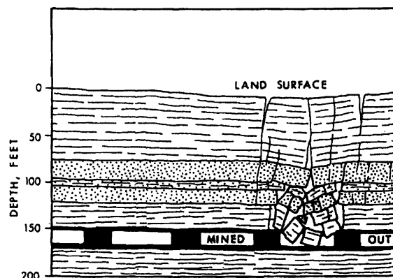
Figure 2. Effect of Mine Roof Collapse Resulting From Room and Pillar Mining.
